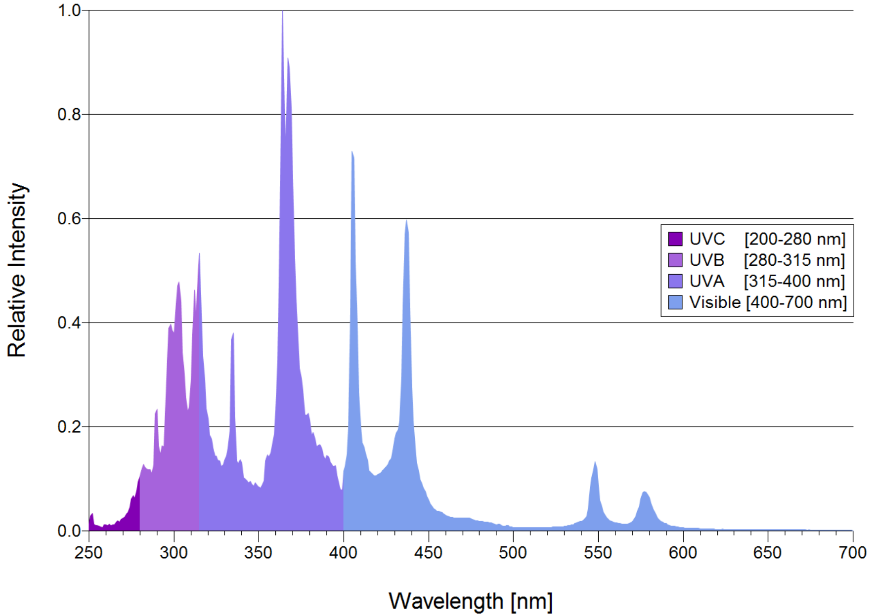
Uvitron 200W UVB Enhanced Spot Lamp Spectral Distribution UV2170
