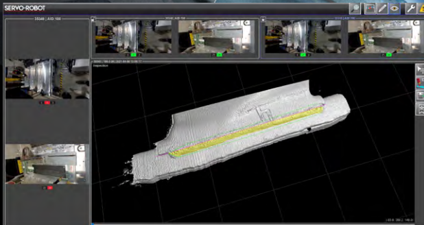
Example of weld surface map created by the Vision System
