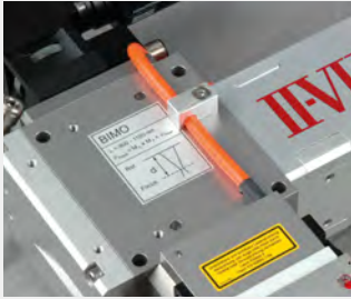
Process monitoring module for CCTV-viewing and/or 90° beam bending
