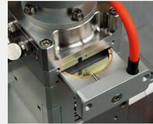
Cover slide for additional protection of collimation
