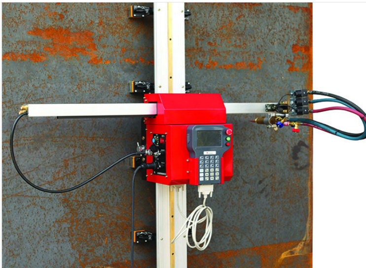
Portable CNC Cutting Machine (/portable-cnc-cutting-machine-46.html)
