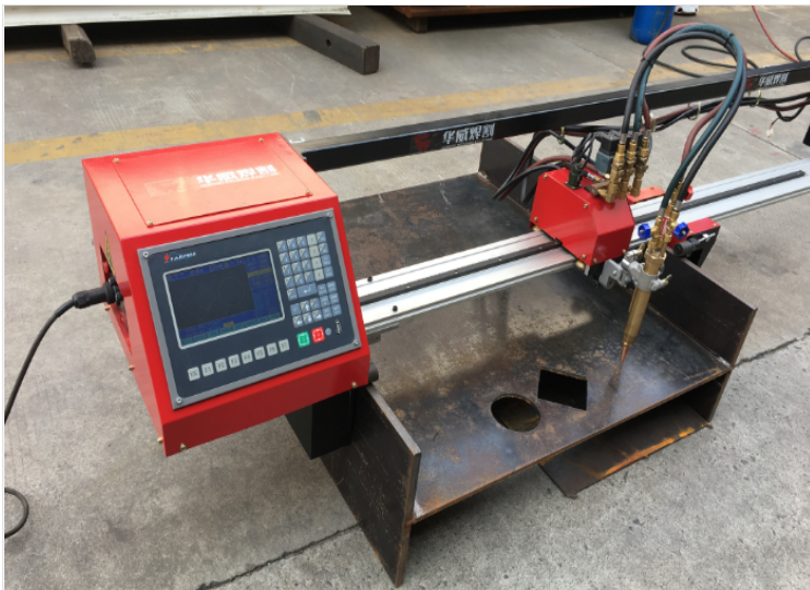
Portable CNC Cu (/portable-cnc-cutting-machine-46.html)
