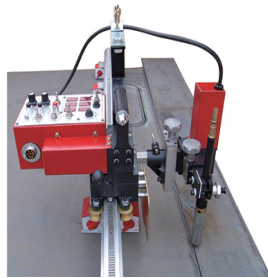
(/hk--magnetic-straight-welding-swing-model-oscillation-auto-weld-carriage-166.html) HK-100 Magnetic Straight Welding Swing Mod...
