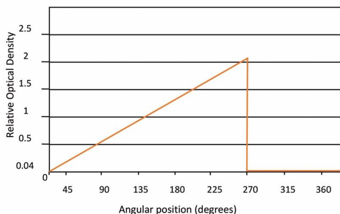
Circular Variable ND Filter
