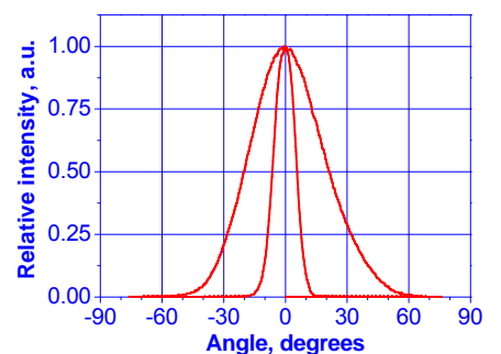
Far field (20 mW)
