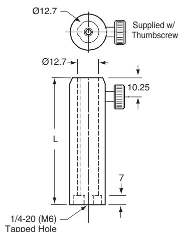
Half-inch Post Holder
