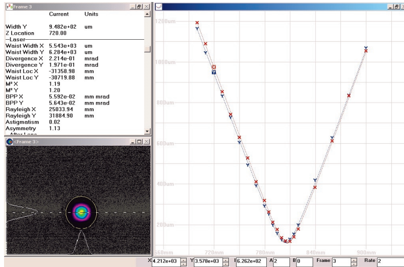
Phidia-c-1 Output Beam Quality Measurement
