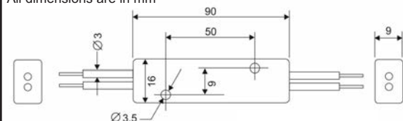
Figure 2: Dimensions of 1x2 or 2x2 Fused Splitter With 3mm Cabled Fibers
