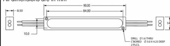
Figure 3: Dimensions of 1x2 or 2x2 Fused Splitter With 3mm Cabled Fibers (Version 2)
