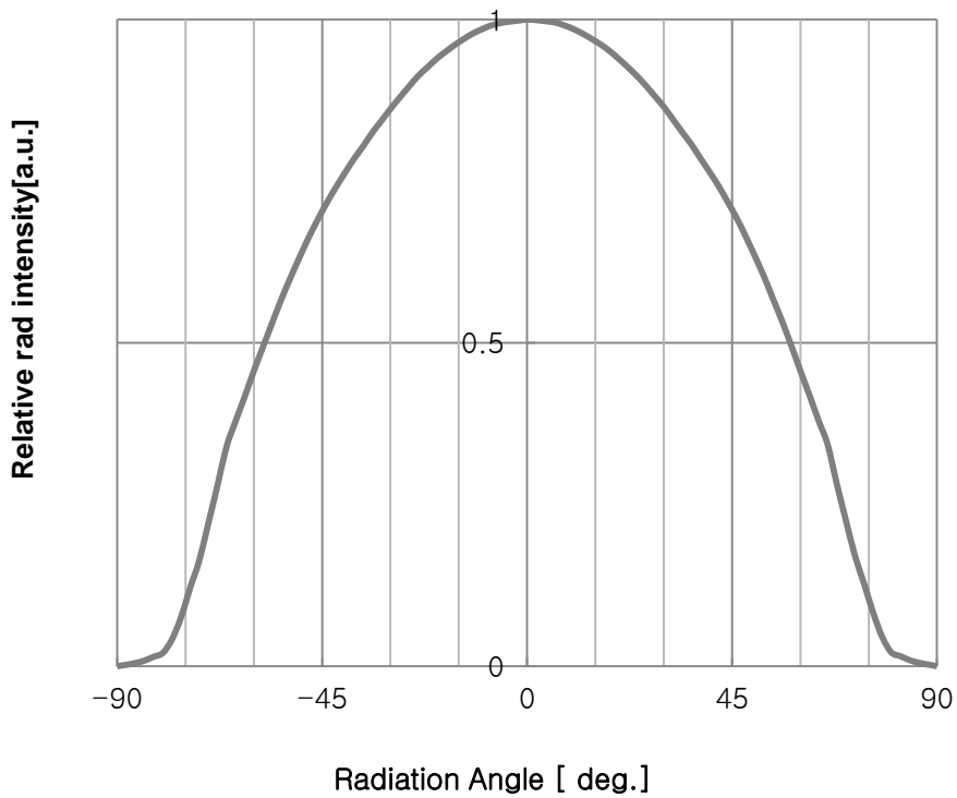
Fig 8. Typical Spatial Distribution, I_F=2A
