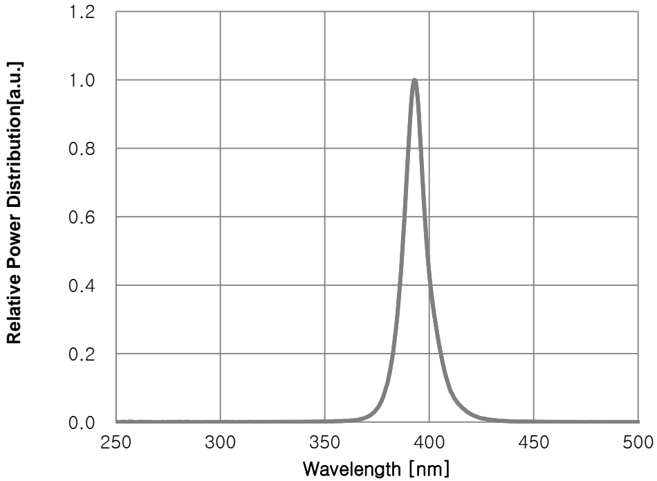
Fig 1. Spectrum, T_a=25^\circ\text{C} , I_F=9\text{A}
