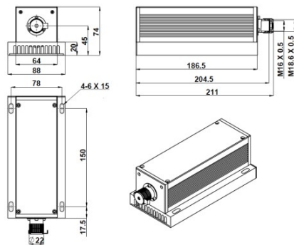
211 (L)×88(W)×74(H) mm 3 , 1.6 kg
