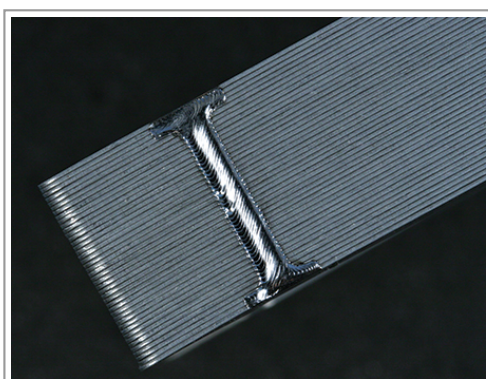
High-speed laser pattern welding
