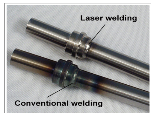
Heat-affected zones Laser welding vs. conventional welding
