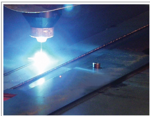
Laser welding with CO2 laser
