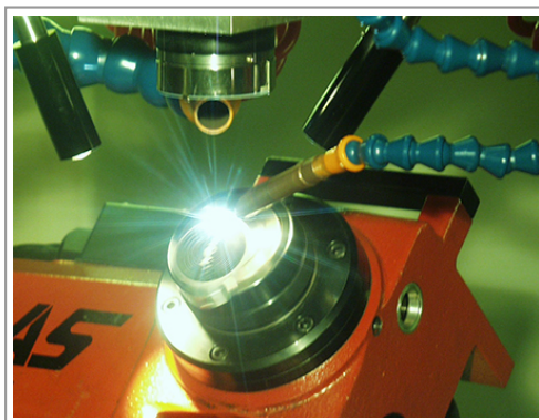
Laser welding with Nd:YAG laser
