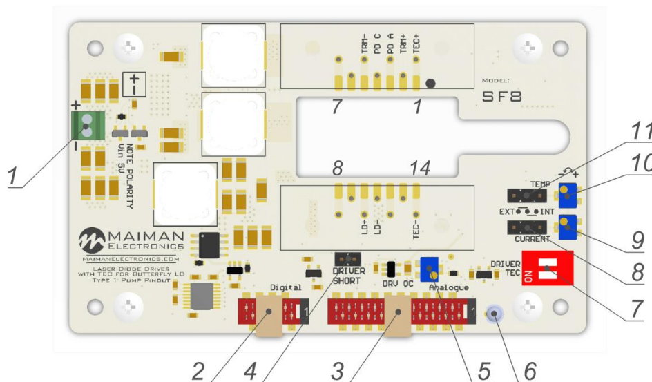
Fig. 7 – Controls
