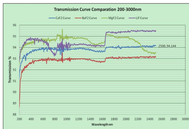
Different wavelength transmission curve compare:(100-200nm, 200-3000nm, 1500-21500nm)
