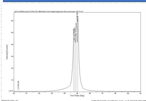
4. LiF material poly/mono x-ray curve
