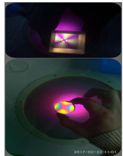
3. MgF2 mono material by polarizing interferometer
