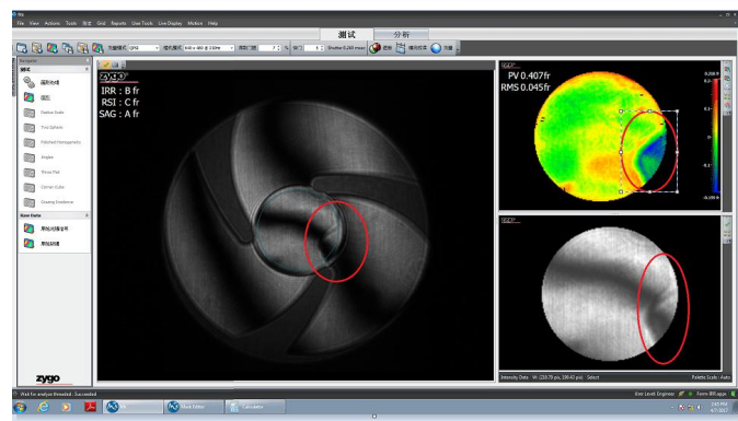
5. CaF2 Mono material by ZYGO
