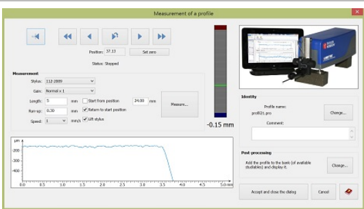
Intra Touch can measure interrupted surfaces
