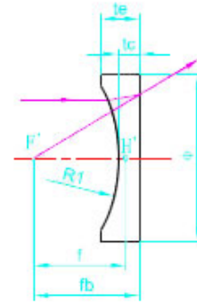
Plano-Concave Lenses
