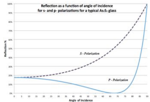
Figure 1: Reflection as a function of incident angle for S- and P-polarizations for an air-to- As_2S_3 interface. It can be seen that for a certain angle the P-polarization experiences 0% reflection.
