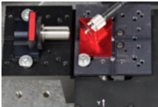
Figure 3: Setup for coupling into the FC/B ® connector end using the FC/B ® holder
