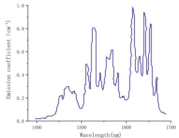
Emission
