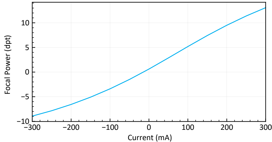
Figure 6: Typical data showing the relation between focal power (in diopters) and electrical current
