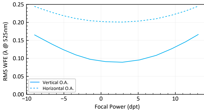
Figure 8: Typical wavefront error of the EL-12-30-TC vs focal power with optical axis vertical and horizontal (@525nm, measured over 80% of the clear aperture).
