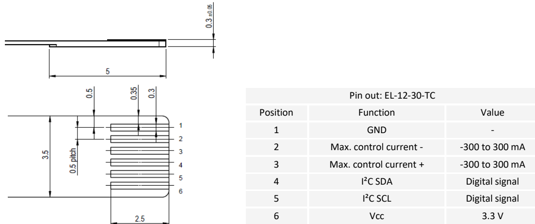
Figure 3: Electrical flex connections of the EL-12-30-TC
