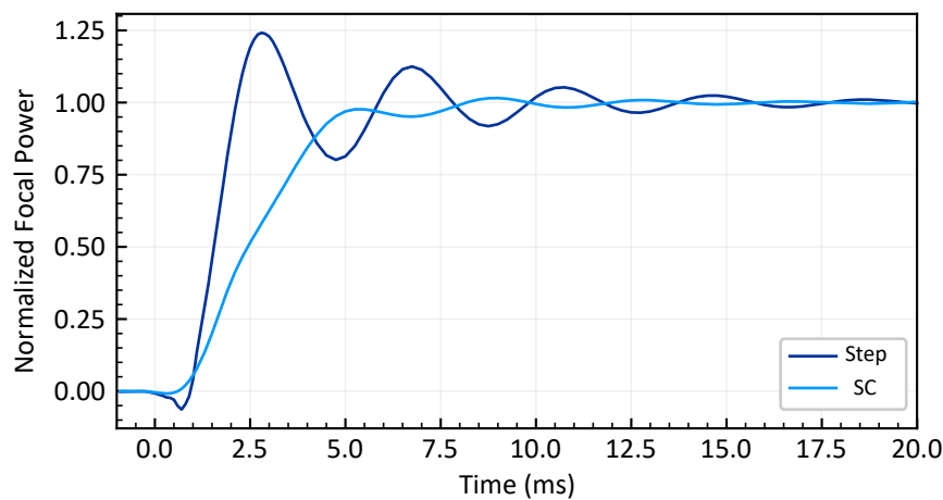
Figure 9: The settling time can be improved with signal conditioning (SC)
