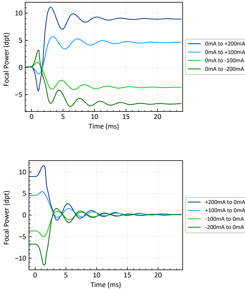
Figure 10: Typical focal power response of the EL-12-30-TC. The upper plot shows a series of steps from low to high current and the lower plot for steps from high to low current.
