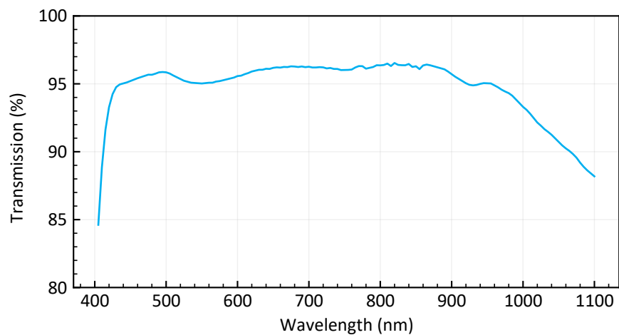
Figure 7: Transmission spectrum of standard EL-12-30-TC.
