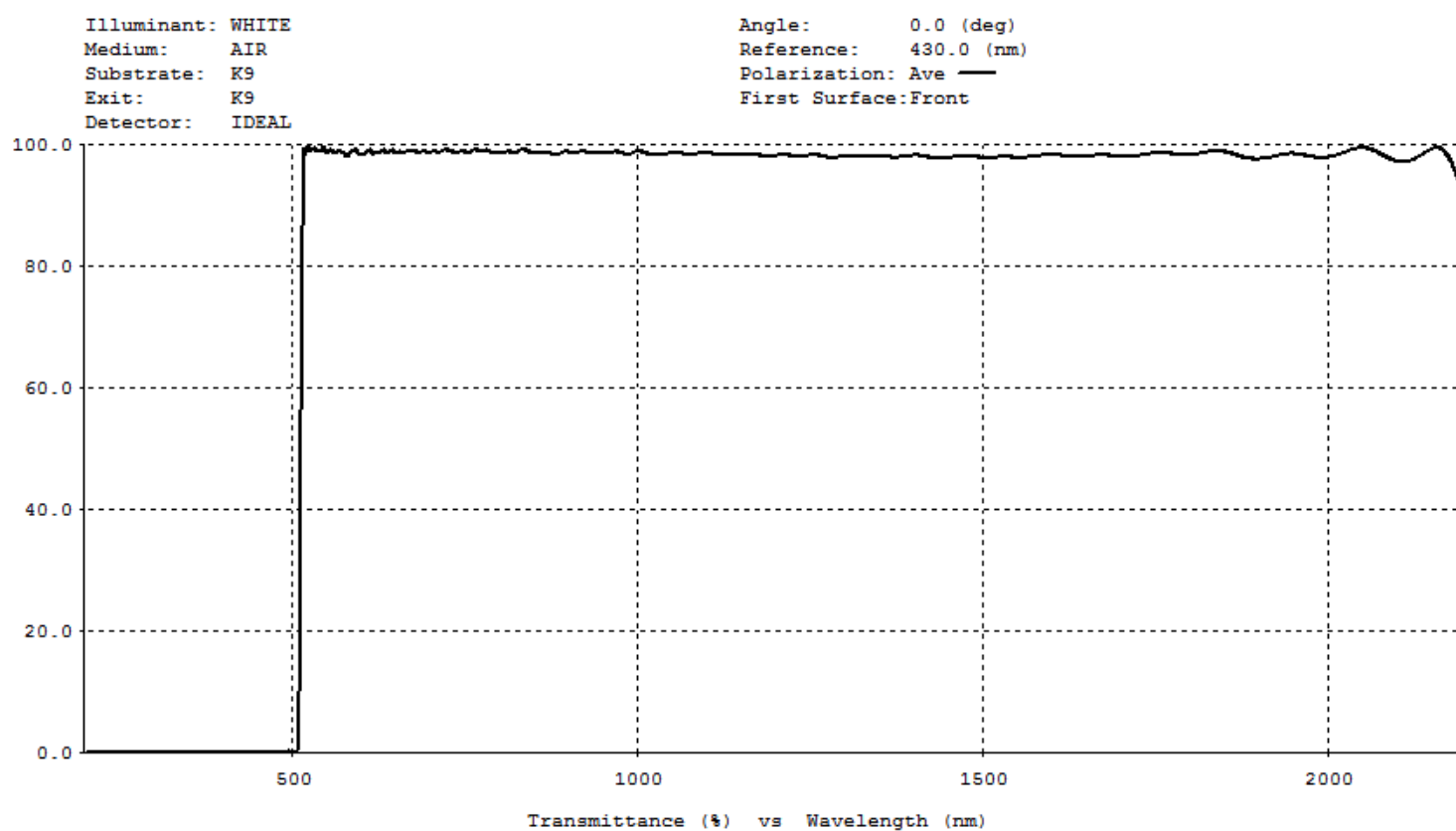
HT@508-2150nm & HR@200-492nm AOI=0°
