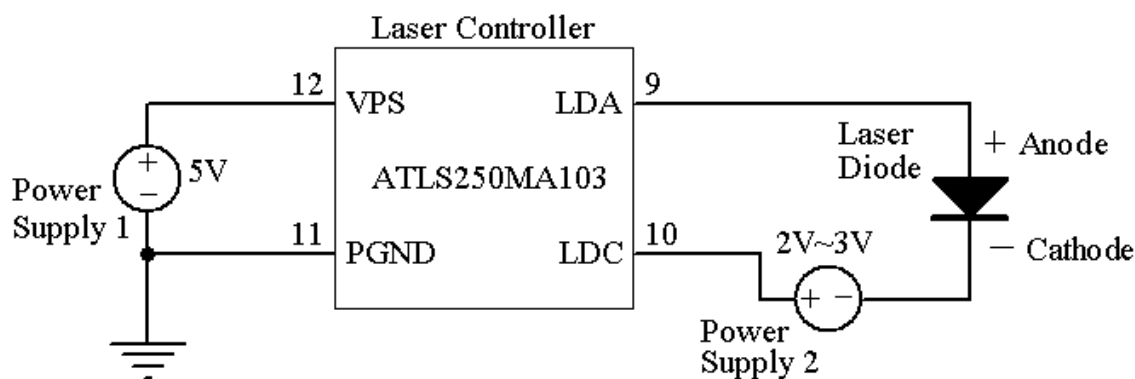
Figure 7. Driving High Voltage Laser Diodes
