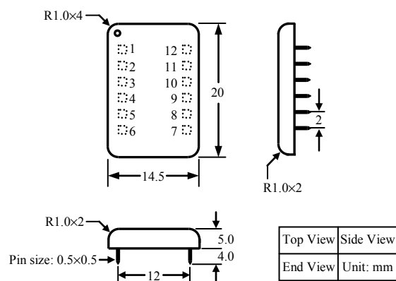
Figure 8. Dimensions of the DIP Package Controller
