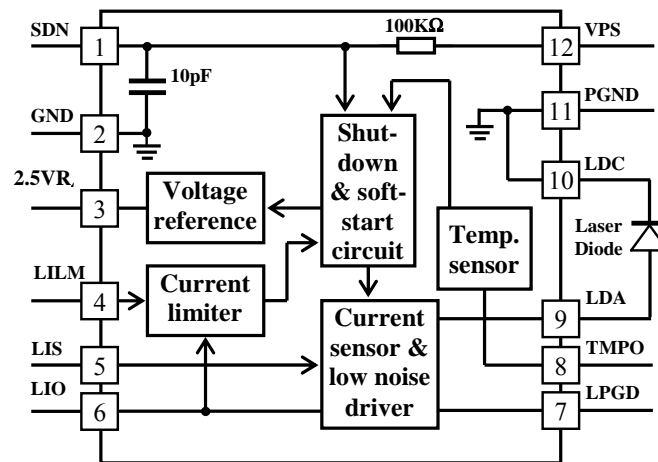
Figure 3. Block Diagram
