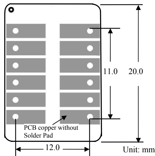
Figure 11.1. Top View of the Bottom Side of the Recommended PCB Foot-print
