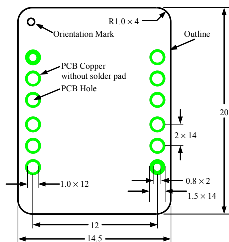
Figure 10. Top Side PCB Foot-print for the DIP Package
