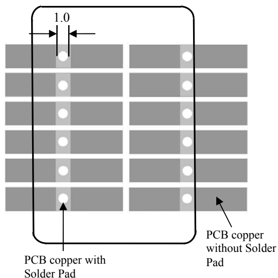
Figure 11.2. Top View of the Bottom Side of the recommended PCB Foot-print
