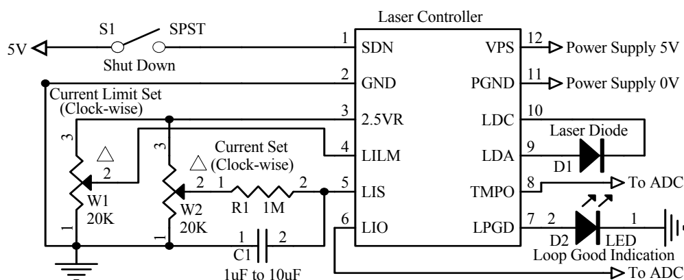
Figure 4.2. Typical Stand-alone Application Schematic for ATLS250MA103-PD
