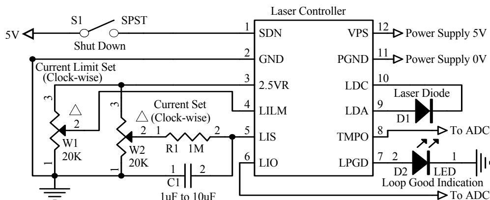
Figure 4.2. Typical Stand-alone CW Operation Schematic for ATLS200MA103-PD
