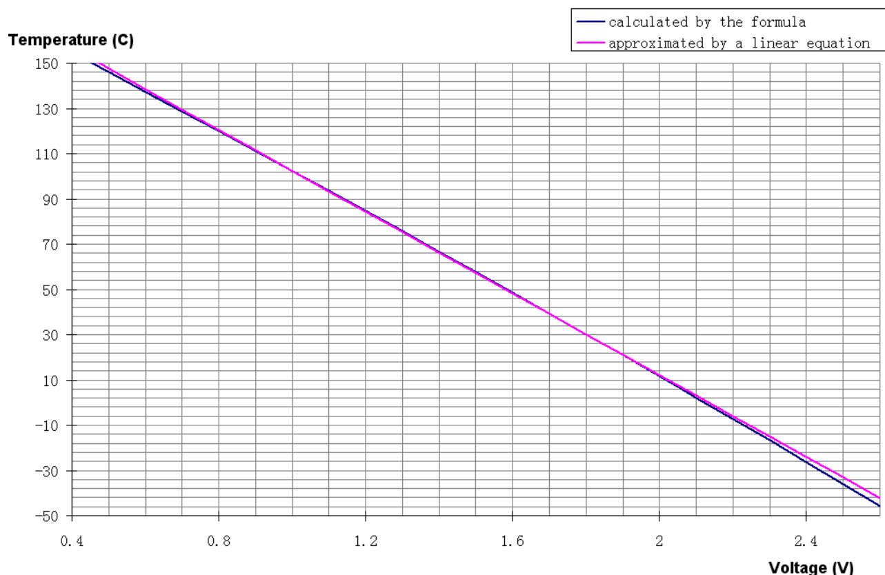
Figure 13. Controller Internal Temperature vs. TMPO Voltage
