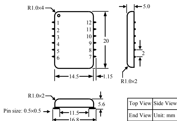
Figure 9. Dimensions of the DIP Package Controller
