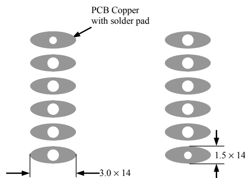
Figure 12. Top View of the Bottom Side PCB Foot-print
