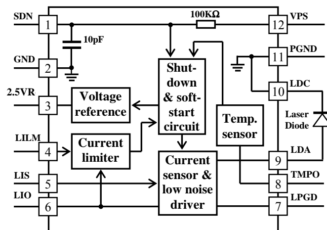
Figure 3. Block Diagram
