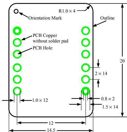
Figure 16. Top Side PCB Foot-print for the DIP Package
