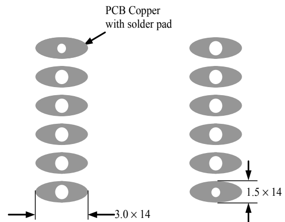
Figure 17. Top View of the Bottom Side PCB Foot-print
