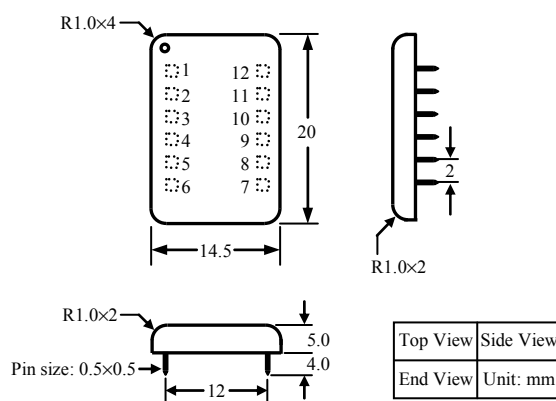
Figure 14. Dimensions of the DIP Package Controller
