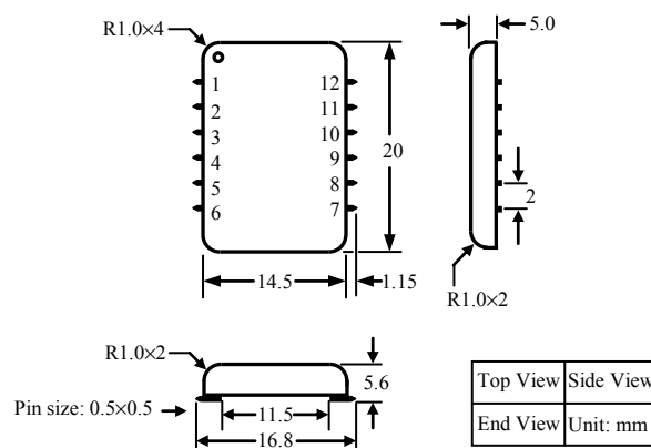
Figure 15. Dimensions of the SMT Package Controller
