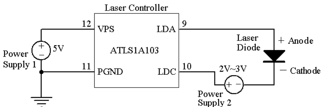
Figure 13. Driving High Voltage Laser Diodes
