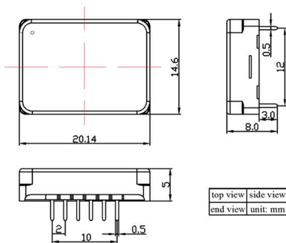
Figure 9. Dimensions of the DIP Package Controller
