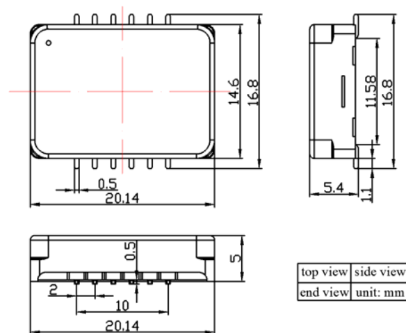
Figure 10. Dimensions of the SMT Package Controller
