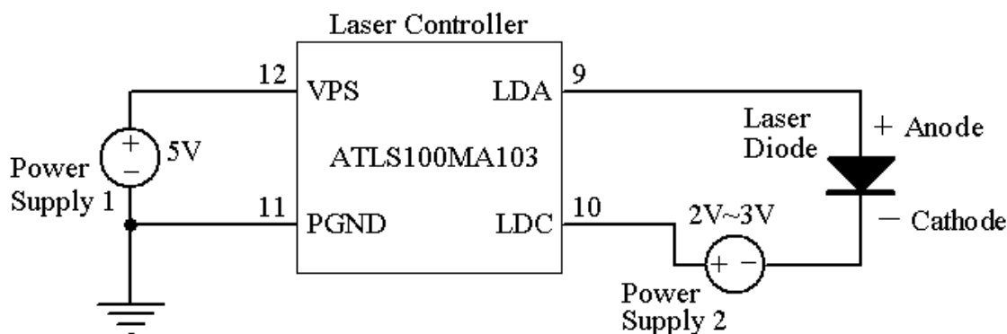
Figure 8. Driving High Voltage Laser Diodes
