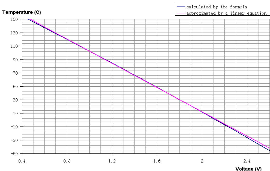
Figure 13. Controller Internal Temperature vs. TMPO Voltage
