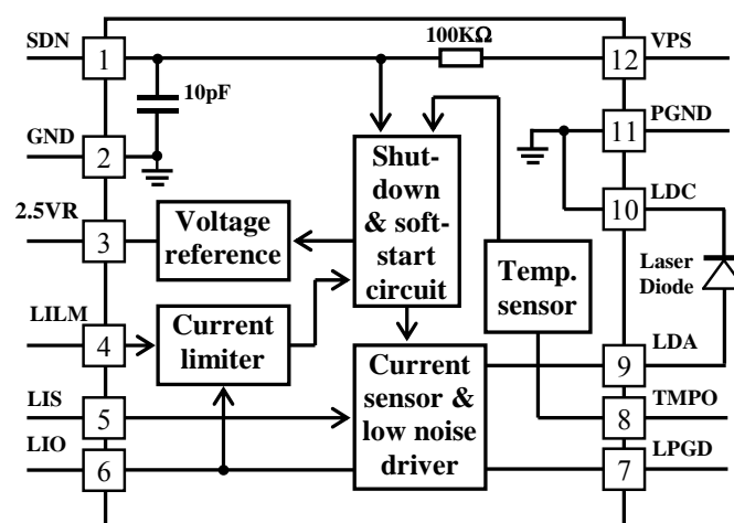
Figure 3. Block Diagram
