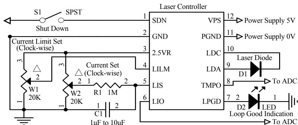
Figure 4.2. Typical Stand-alone CW Operation Schematic for ATLS500MA103-PD
