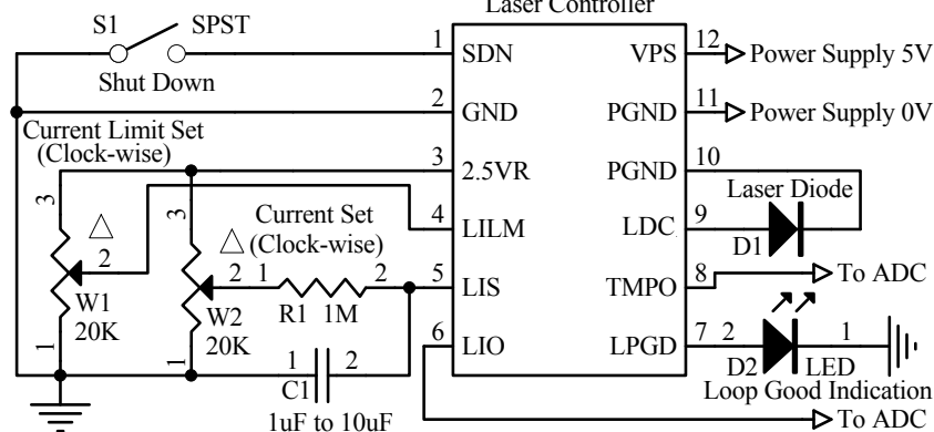
Figure 4.1 Typical Stand-alone CW Operation Schematic for
