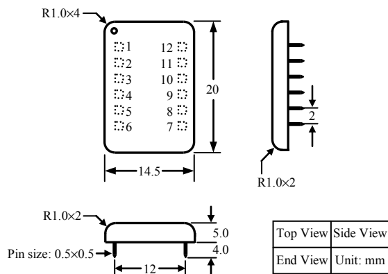
Figure 9. Dimensions of the DIP Package Controller
