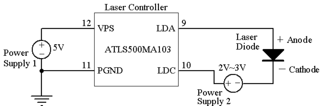
Figure 8. Driving High Voltage Laser Diodes
