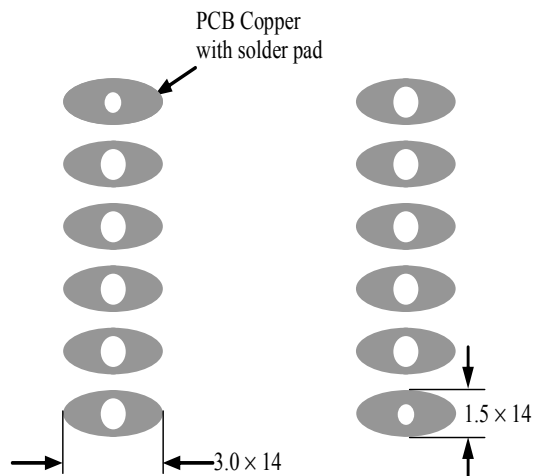
Figure 12. Top View of the Bottom Side PCB Foot-print
