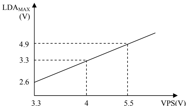
Figure 6. Relationship between VPS and LDA MAX
