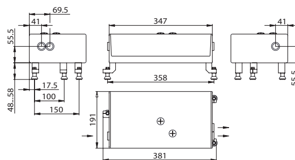
The FG130 harmonic generator outline drawing.
