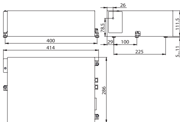
The FX200 laser head outline drawing.
