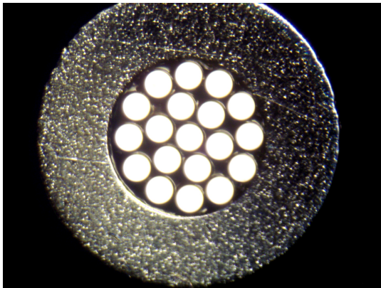
Close up of SMA-905
