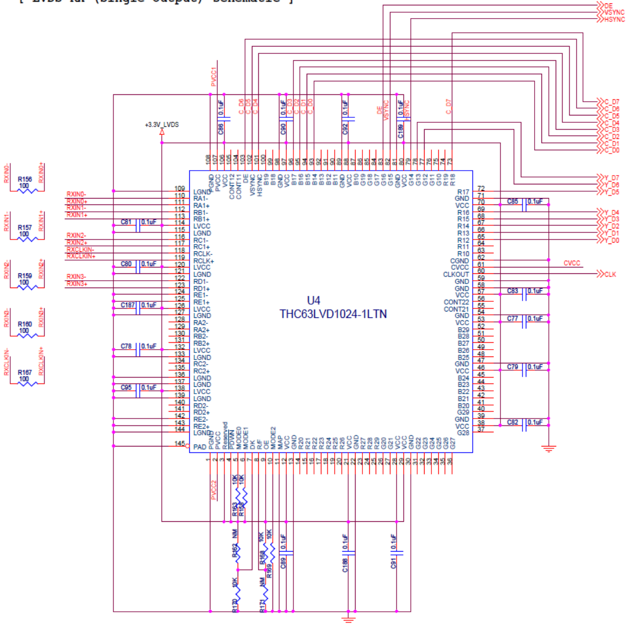
[ LVDS RX (Single Output) schematic ]
