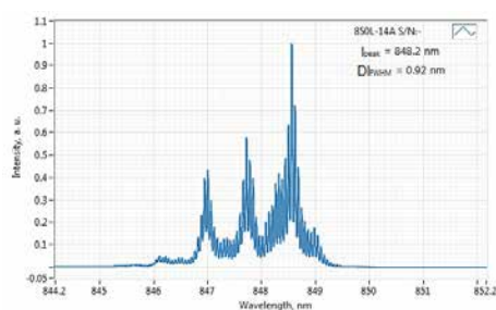
Typical spectrum of 0850 nm diode laser. Measured with 20 pm resolution.
