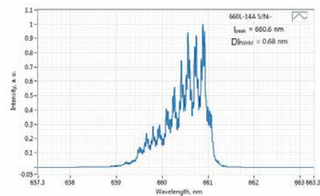
Typical spectrum of 0660 nm diode laser. Measured with 20 pm resolution.
