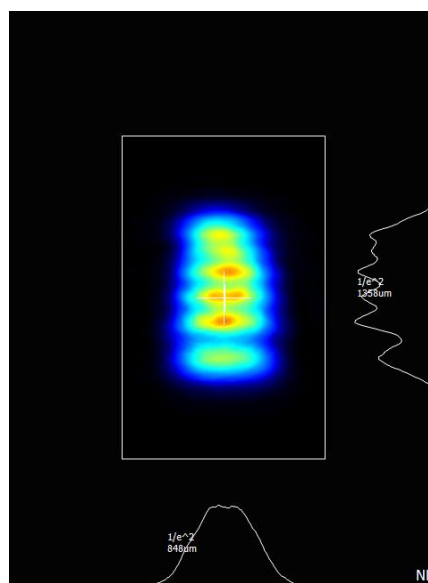
Typical near field (0.45 m from output aperture) beam profile. Non-circularized beam of a 0520 nm direct diode laser.
