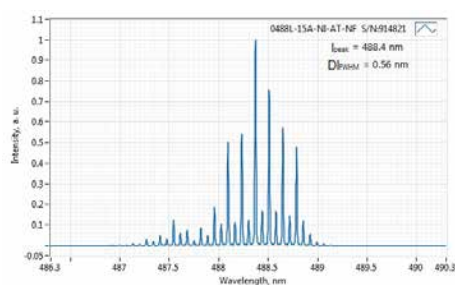
Typical spectrum of 0488 nm diode laser. Measured with 20 pm resolution.
