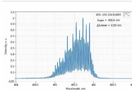
Typical spectrum of 0405 nm diode laser. Measured with 10 pm resolution.
