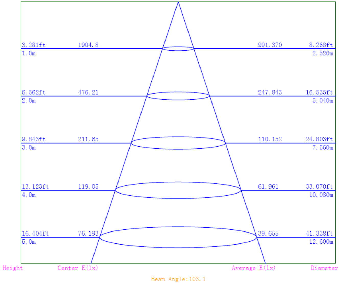
Illuminance-Distance Curve
