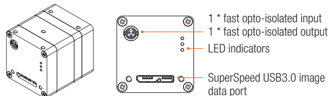
Housed cameras with Micro-B connector
