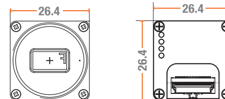
Semi housed cameras with 'FL' ribbon cable connector
