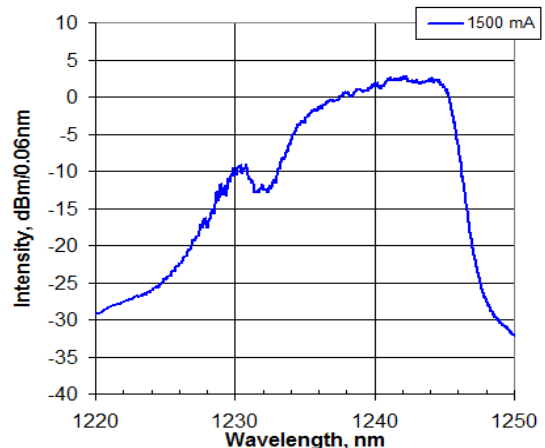
Spectral Characteristics
