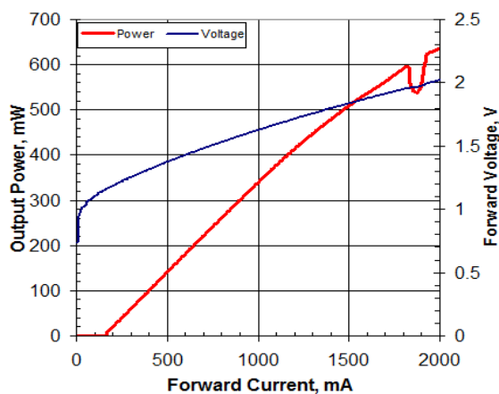
Light-Current-Voltage Characteristics
