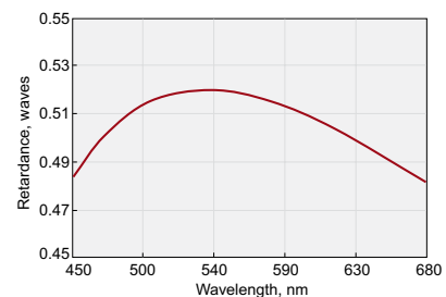
\lambda/2 @ 450-680 nm
